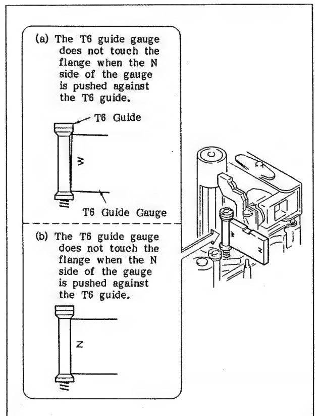
Fig. 6-124 Adjustment of the T6 Guide Roller
